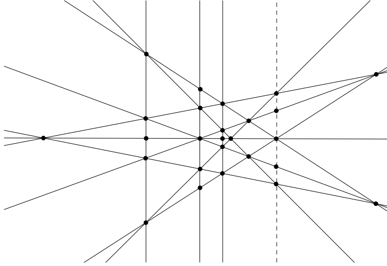
FIGURE 6. The dual of the McKee configuration: 13 lines with 6 double points, 18 triple points and 3 quadruple points (one of which is at infinity, in the direction of the vertical lines).
