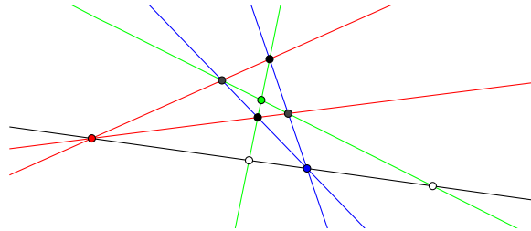
FIGURE 2. Three reducible conics (colored red, green and blue) through 4 general points (the black dots) with an additional line (black) define a configuration of 9 points.
