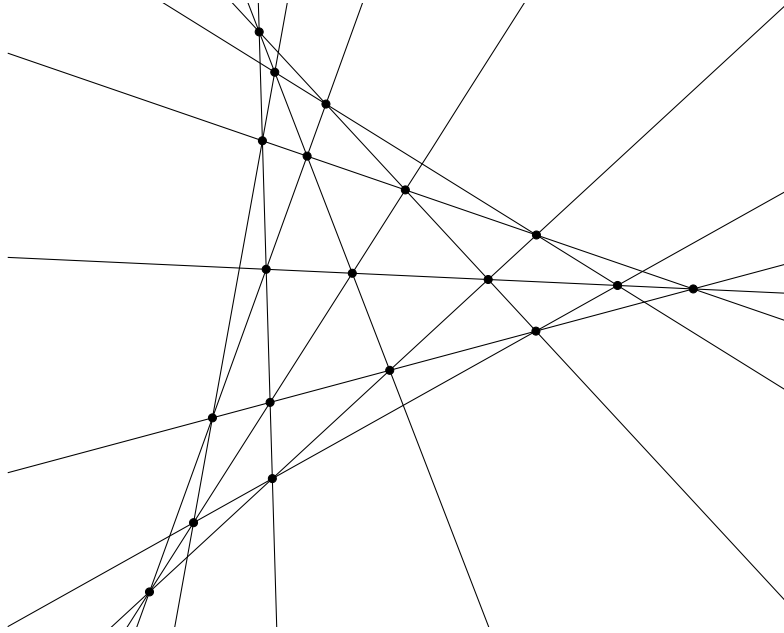
FIGURE 5. A configuration of 12 lines with 19 triple points (and 9 double points).
