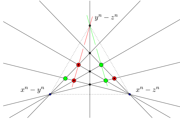
FIGURE 1. The Fermat configuration of 3n complex lines and their n^2 + 3 points of intersection (indicated by filled in circles) for n = 3 . (The coordinate axes are represented by dotted lines. At each coordinate vertex there occur n of the 3n lines, defined by the forms shown; the n^2 + 3 points consist of a complete intersection of n^2 points plus the 3 coordinate vertices. This configuration does not exist over the reals: one must regard the open green circles as representing collinear points, and likewise the dotted red circles as representing collinear points.)
