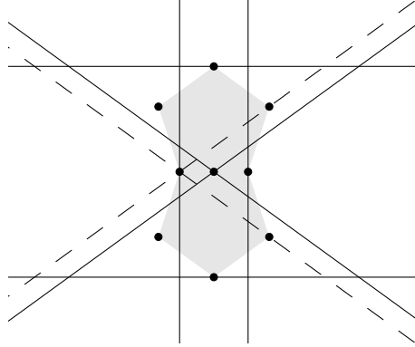
FIGURE 7. The McKee configuration is based on two abutting regular pentagons. It has n = 13 points (including 4 at infinity in the directions of the lines) having only 6 ordinary lines (i.e., less than n/2 lines through exactly two points of the configuration, shown as solid lines; note that the solid diagonal lines are parallel to the dashed lines).
